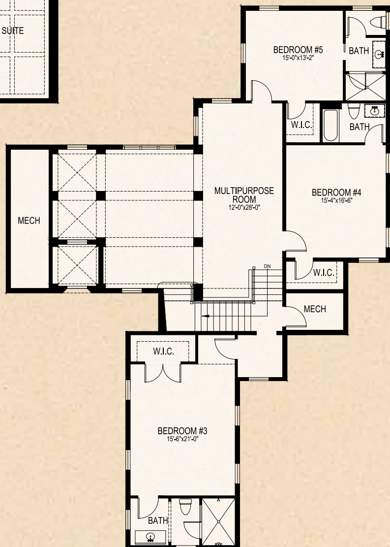
SECOND FLOOR
